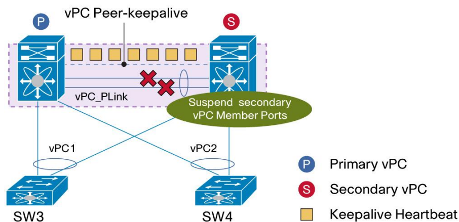
Figure 11. vPC Peer-Link Failure - Behavior On Secondary Peer Device
