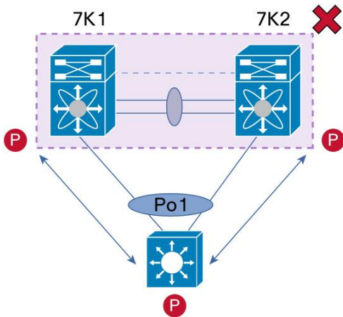
Figure 60. Layer 3 and vPC Unsupported Designs: Peering Over a vPC Interconnection
