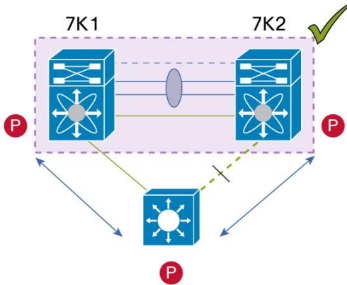
Figure 54. Supported Designs for Layer 3 and vPC: Peering over a Spanning Tree Protocol Interconnection Using a non-vPC VLAN
