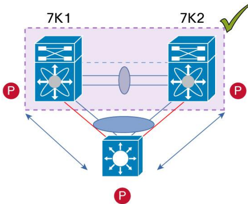
Figure 56. Layer 3 and vPC Supported Designs: Peering with an External Router on Parallel Interconnected Routed Ports
