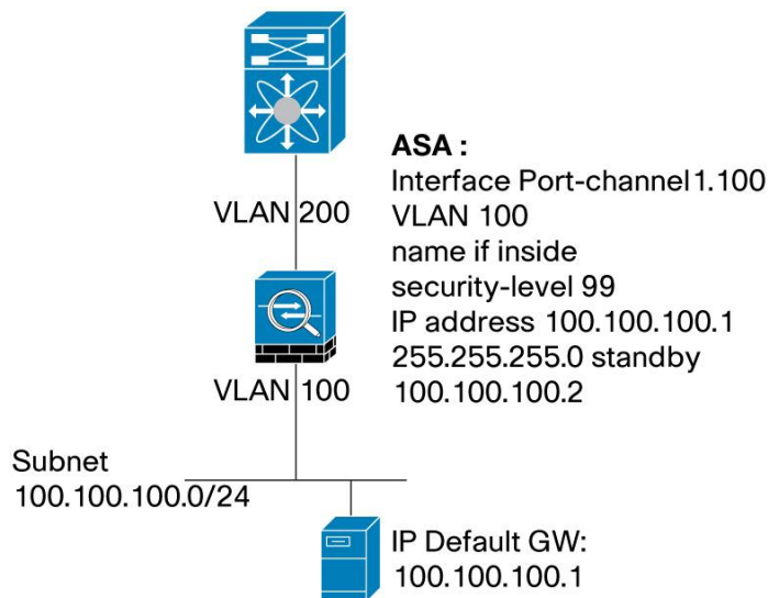
Figure 77. ASA in Routed Mode Connected to vPC Domain - Logical View
