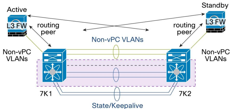
Figure 75. Service Appliance in Routed Mode Connected to vPC Domain Using Single Link
