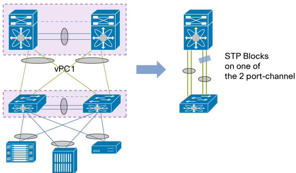
Figure 33. Incorrect Configuration of Double-Sided vPC Topology
