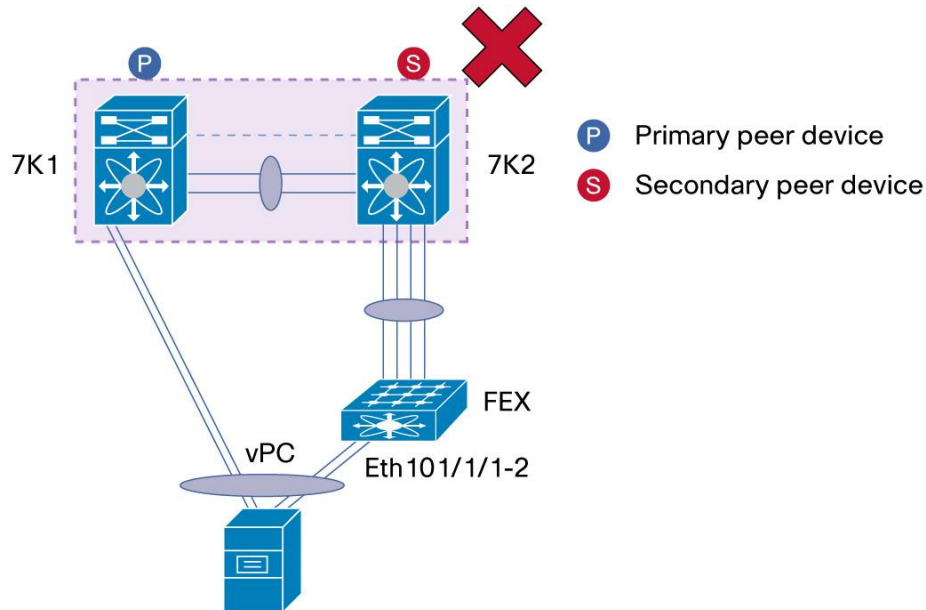
Figure 84. FEX with vPC - vPC with 1 Leg on FEX and the Other Leg On NEXUS 7000 Line Card - Not Supported
