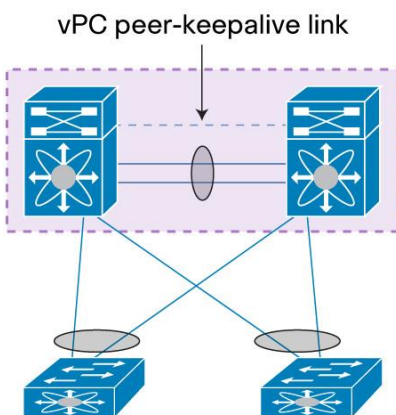
Figure 14. vPC Peer-Keepalive Link
