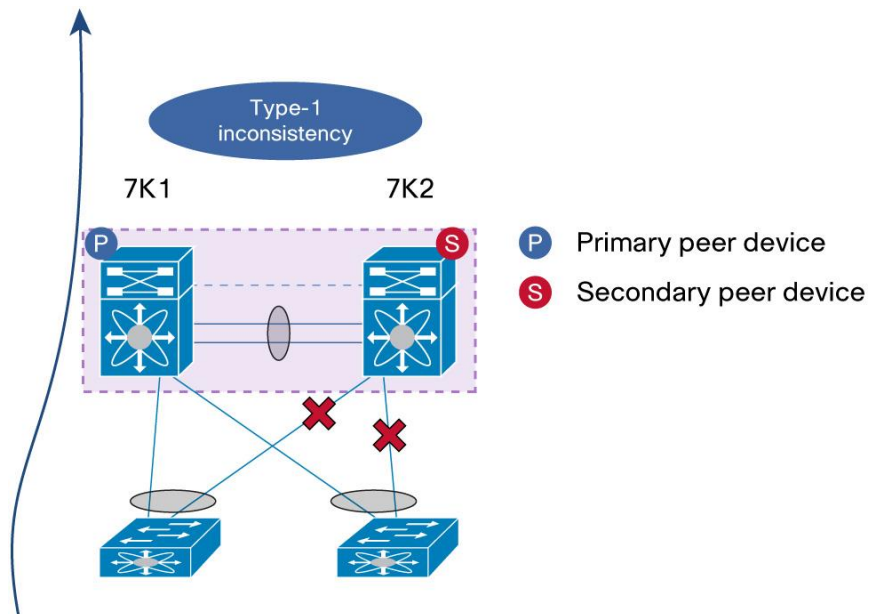
Figure 94. vPC Graceful Type-1 Checks
