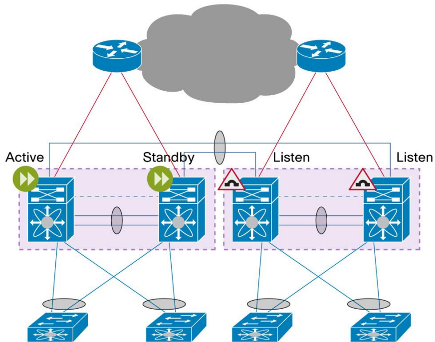
Figure 8. vPC for Data Center Interconnect: Dual Layer 2 /Layer 3 Pod Interconnect
