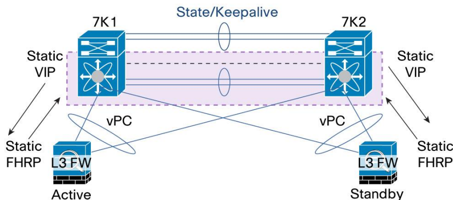
Figure 74. Service Appliance in Routed Mode Connected to vPC Domain Using vPC Link
