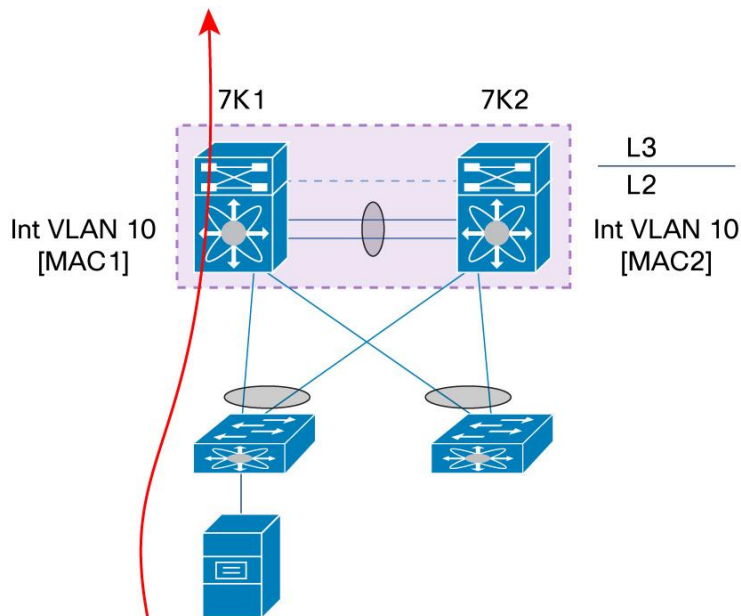
Figure 90. vPC Peer-Gateway
