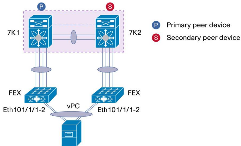
Figure 82. FEX with vPC - Host vPC
