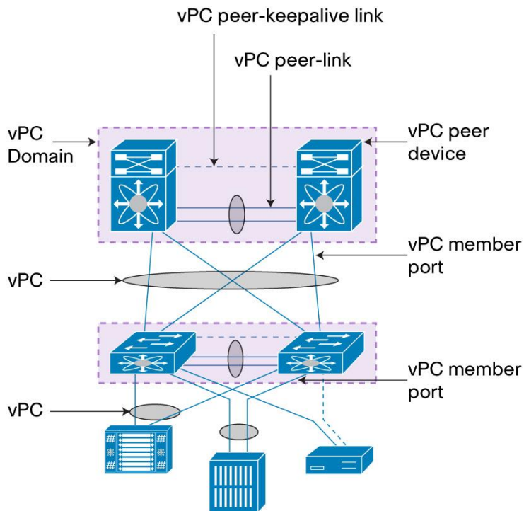
Figure 2. vPC Components
