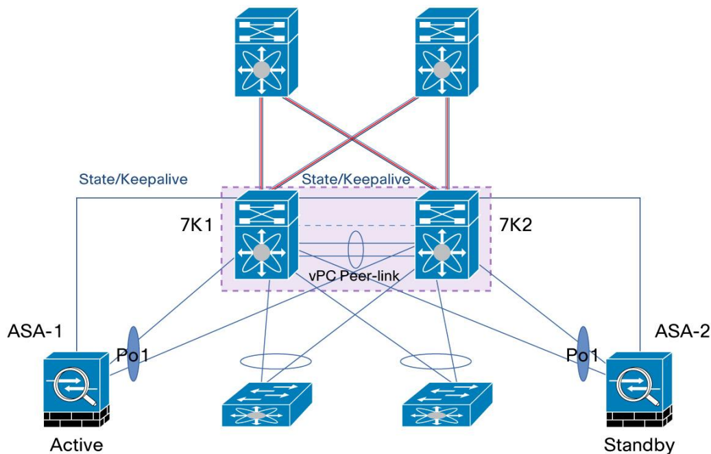
Figure 76. ASA Services Appliance Configured in Routed Mode and Connected to vPC Domain
