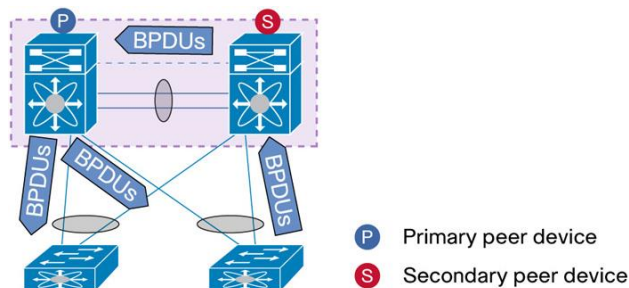
Figure 41. vPC and Spanning Tree Protocol BPDUs
