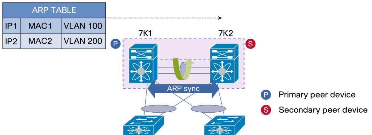
Figure 92. vPC ARP Sync - vPC Peer-Link Fails and Recovers
