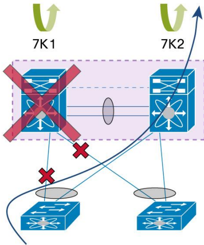
Figure 96. vPC Auto-Recovery Reload-Delay - Both vPC Peer Devices Reload But Only 7K2 Comes Back to Life
