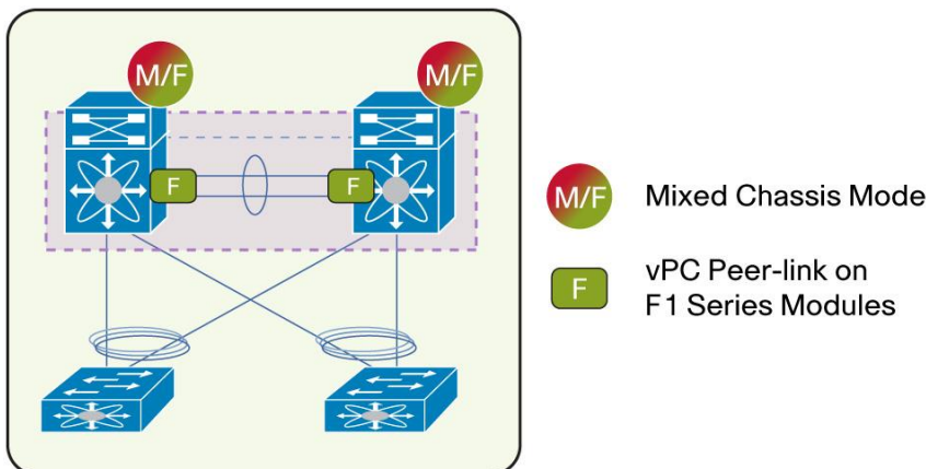
Figure 91. vPC Peer-Gateway Exclude-VLAN - Unique Topology Where the Feature Apply
