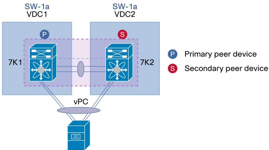
Figure 86. vPC Domain Created Within the Same NEXUS 7000 Chassis Using 2 Different VDC
