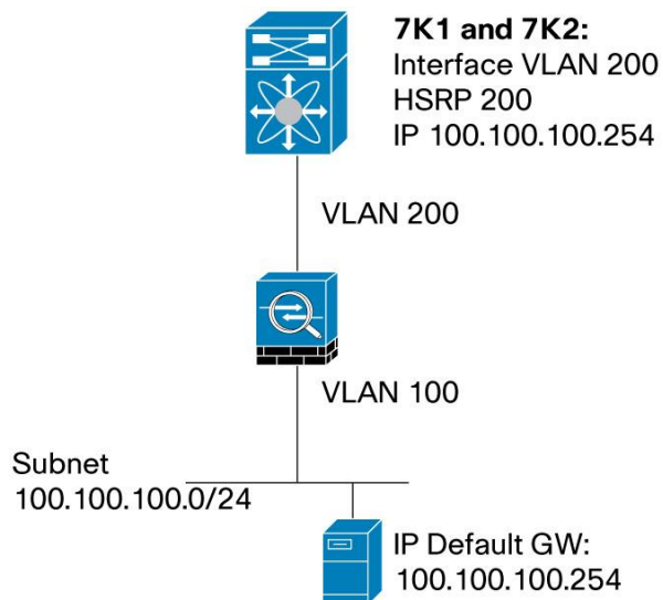
Figure 73. ASA in Transparent Mode Connected to vPC Domain - Logical View
