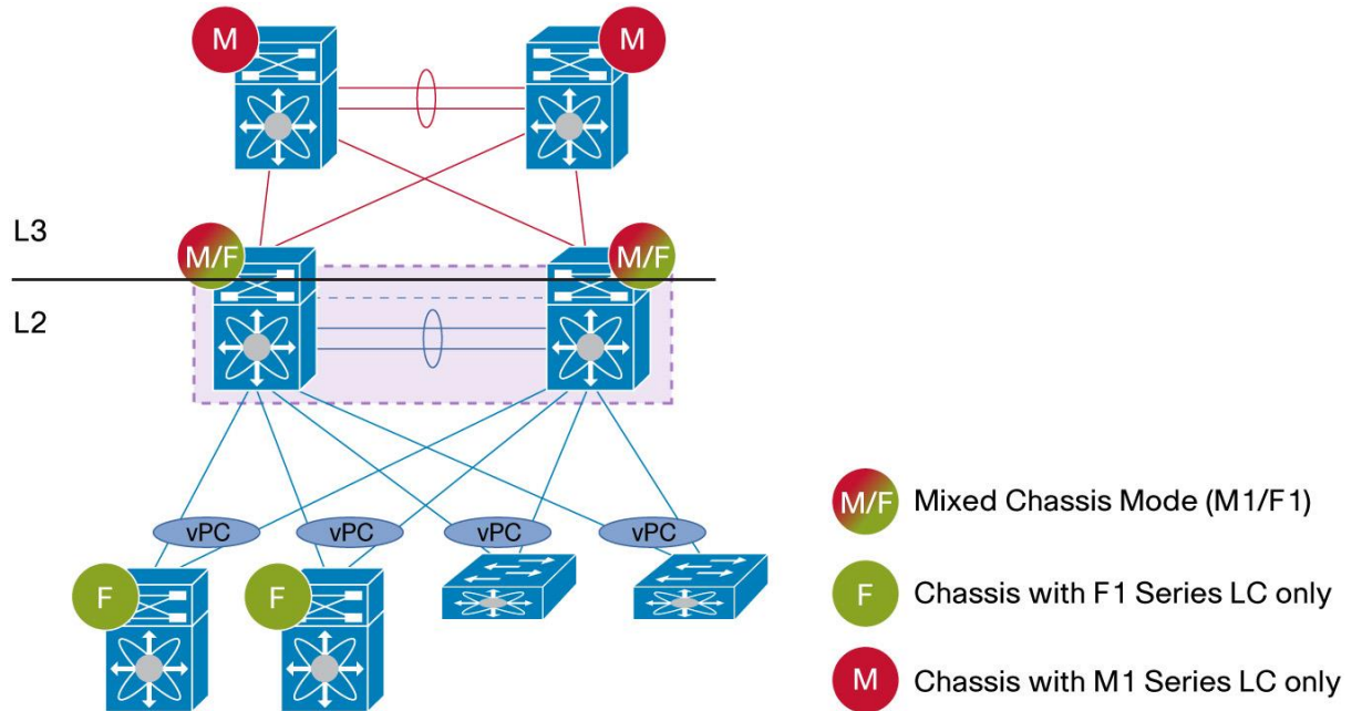
Figure 25. vPC System in Mixed Chassis Mode Configuration
