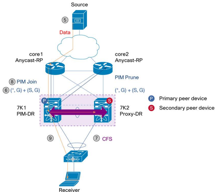
Figure 80. How Multicast Works with vPC (Multicast Packet Flow) - Contd
