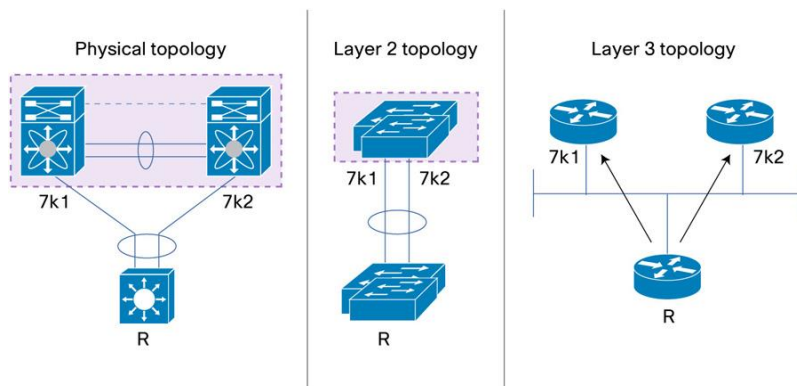
Figure 48. Different Views for vPC Peer Devices Depending on Layer 2 or Layer 3 Vision of the Network
