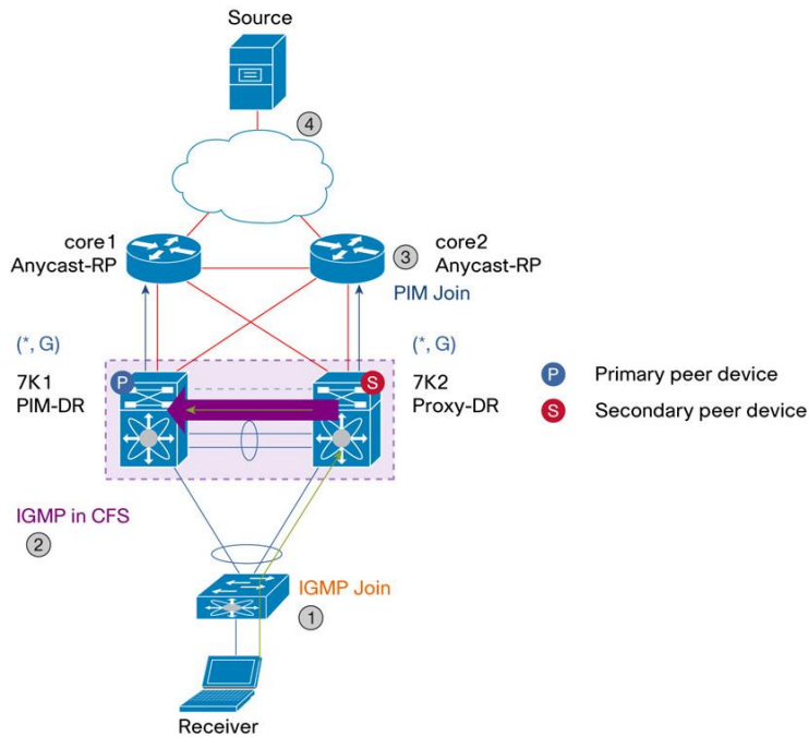
Figure 79. How Multicast Works with vPC (Multicast Packet Flow)
