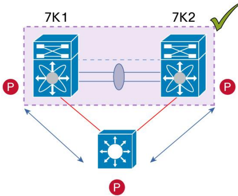
Figure 52. Supported Designs for Layer 3 and vPC: Peering with an External Router Using L3 Links
