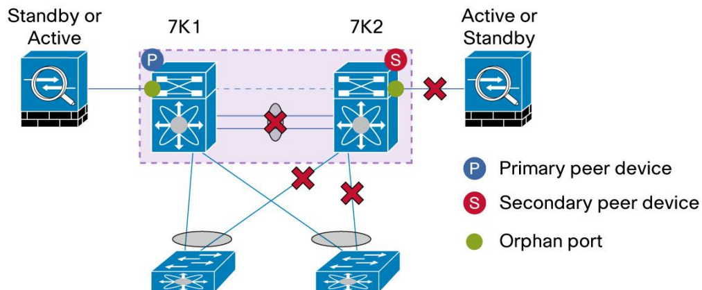
Figure 97. vPC Orphan Ports Suspend
