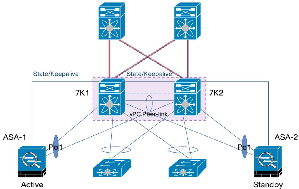
Figure 72. ASA Services Appliance Configured in Transparent Mode and Connected to vPC Domain
