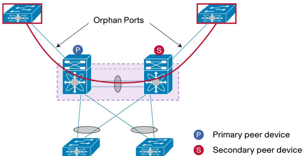
Figure 36. Access Device Single-Attached to vPC Domain Using vPC VLAN
