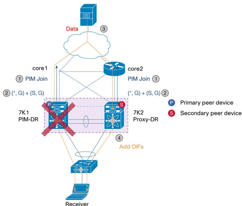
Figure 81. Multicast with vPC - PIM Prebuild SPT
