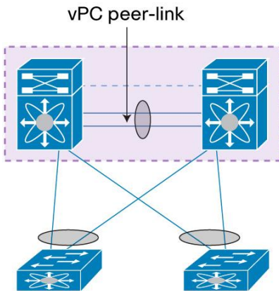
Figure 17. vPC Peer-Link
