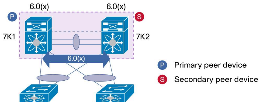
Figure 89. ISSU with vPC - Step 3
