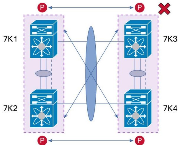
Figure 62. Layer 3 and vPC Unsupported Designs: Peering Over a vPC Interconnection (DCI Case)
