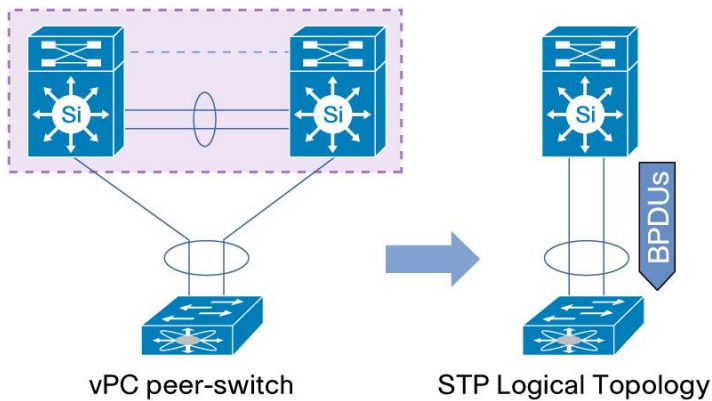
Figure 42. vPC Peer-Switch
