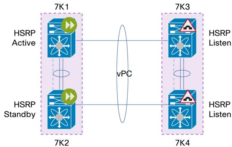
Figure 67. DCI with a Single HSRP/VRRP Group - Active/Active in DC1 and Listen/Listen in DC2
