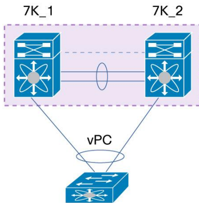
Figure 12. vPC Role and vPC Operational Role
