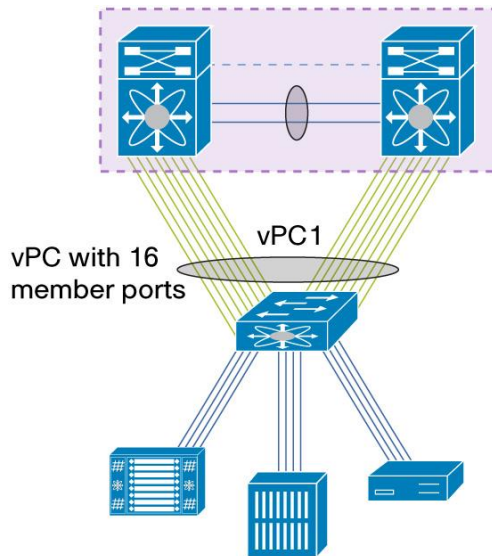
Figure 30. Single-Sided vPC with 16-Way Port-Channel
