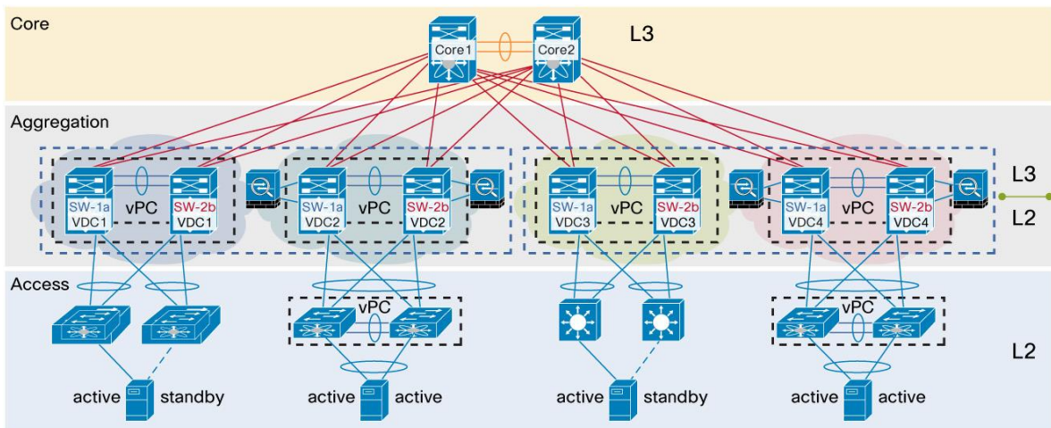
Figure 85. vPC and VDC Interaction - Creating 4 Independent vPC Domains with 2 NEXUS 7000 Series Chassis
