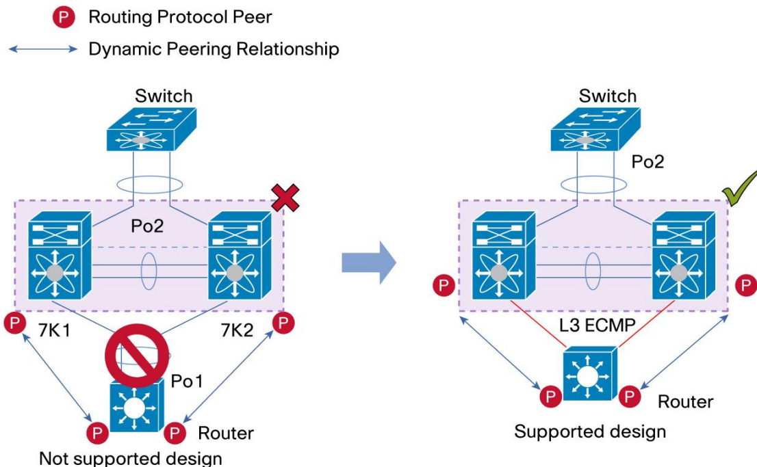
Figure 49. Using Separate Layer 3 Links to Connect L3 Device to a vPC Domain
