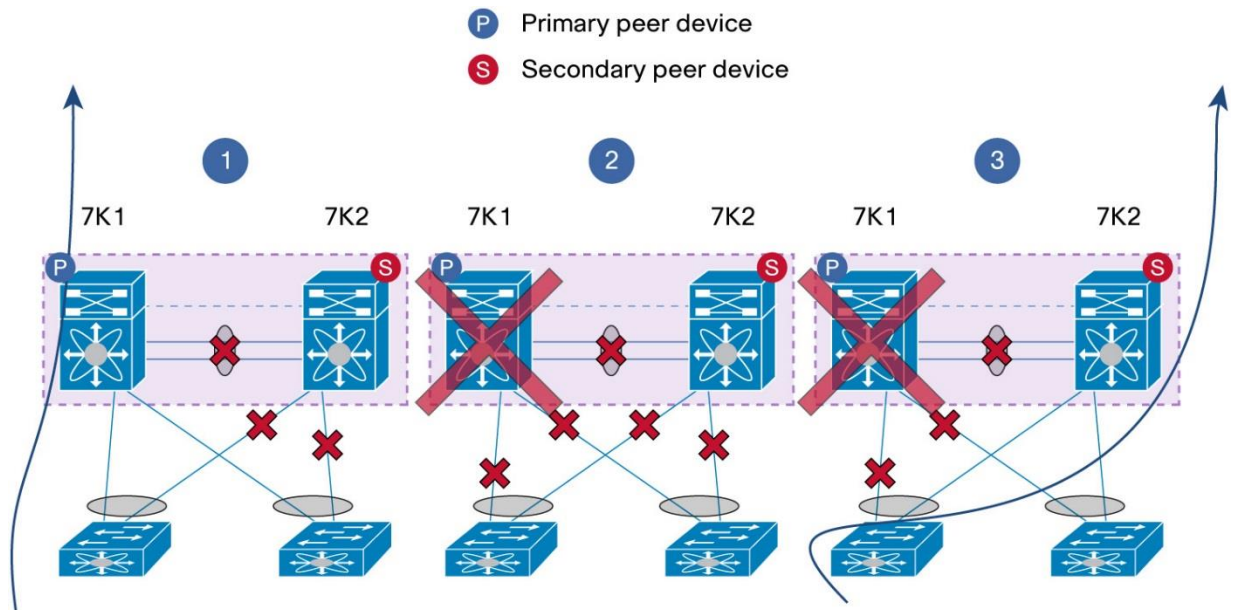
Figure 95. vPC Auto-Recovery - vPC Peer-Link Failure Then vPC Primary Peer Device Failure
