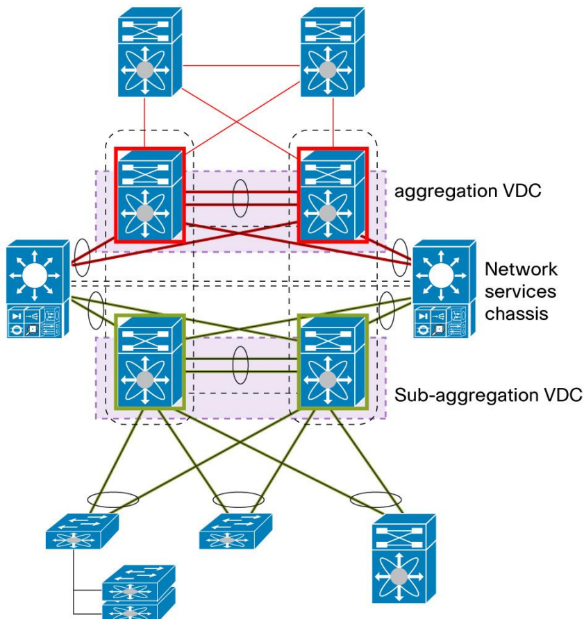
Figure 70. Network Services Chassis with VDC Sandwich Design
