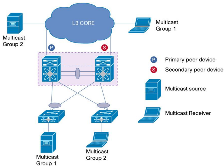
Figure 78. Multicast with vPC
