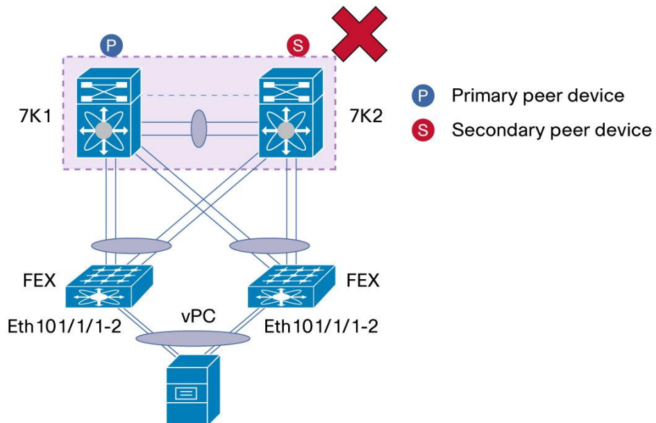
Figure 83. FEX with vPC - eVPC (Enhanced vPC) - Not Supported
