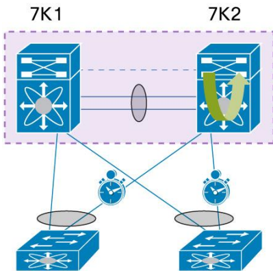
Figure 93. vPC Delay Restore - 7K2 Fails and Then Recovers
