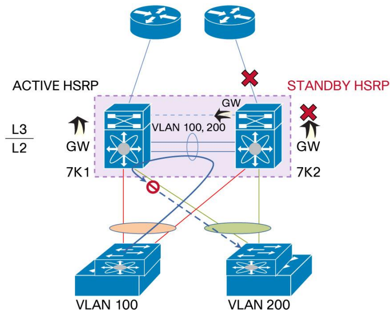
Figure 66. The Problem with HSRP/VRRP Object Tracking in a vPC Configuration
