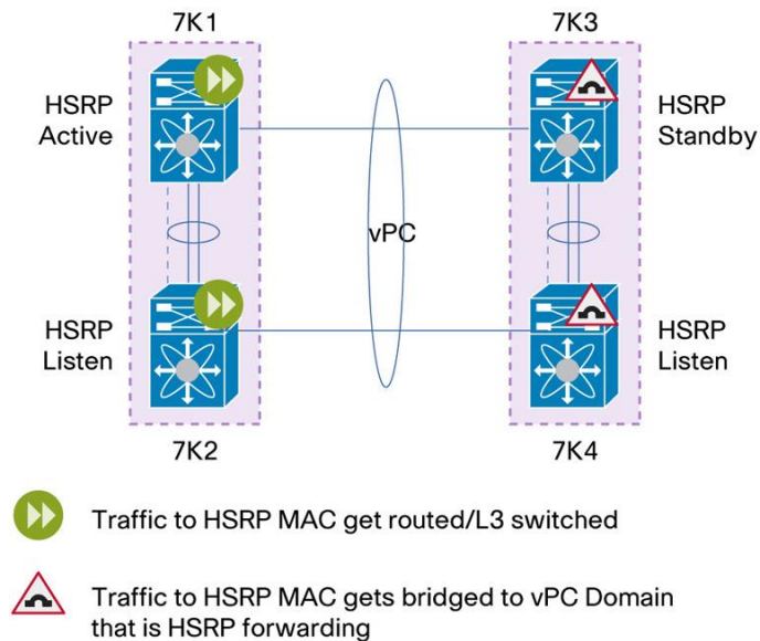
Figure 68. DCI with a Single HSRP/VRRP Group - Active/Active in DC1 and Listen/Listen in DC2
