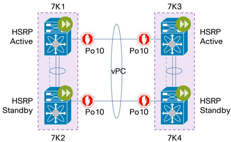
Figure 69. DCI with a Single HSRP/RRP Group - Active/Active in DC1 and Active/Active in DC2
