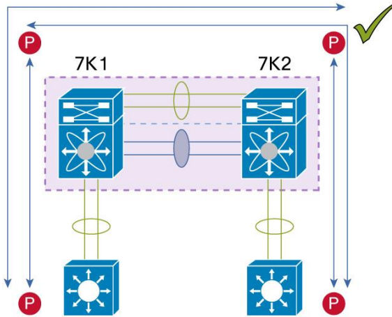
Figure 58. Layer 3 and vPC Supported Designs: Peering over PC Interconnection and Dedicated Interswitch Link Using non-vPC VLAN
