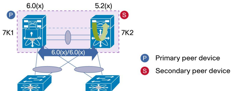
Figure 88. ISSU with vPC - Step 2
