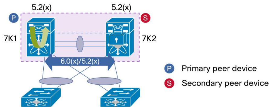
Figure 87. ISSU with vPC - Step 1
